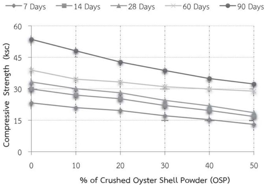
รูปที่ 4 Compressive strength of interlocking block with crushed oyster shell (OSP) at 0, 10, 20, 30, 40 and 50% by the weight of the binder
