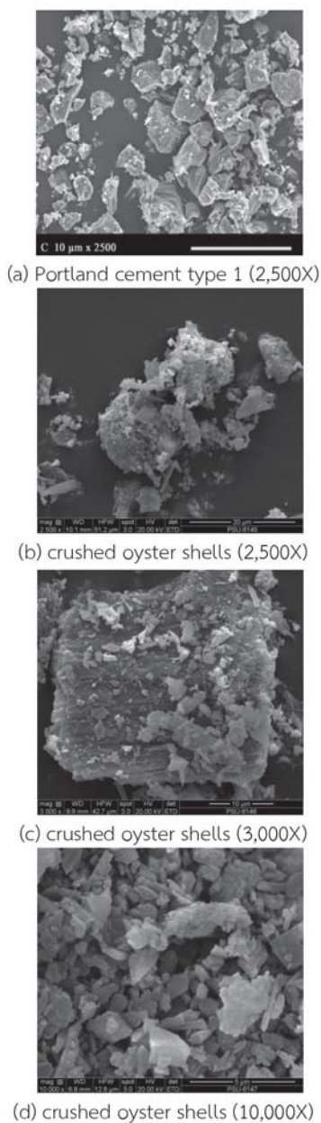
รูปที่ 3 The image of materials from SEM at 2,500, 3,000, and 10,000 magnification
